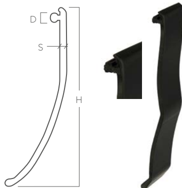
art. 50186522 50186524
